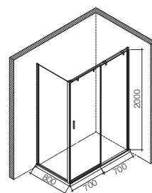
Isometric View
