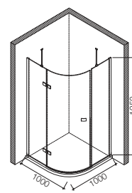
Isometric View
